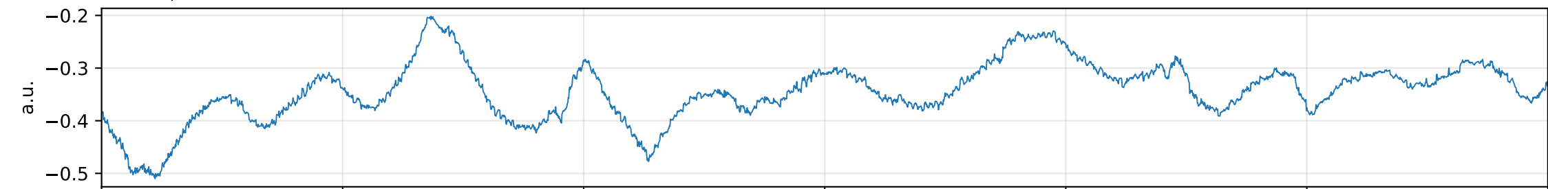
ICA component 1
