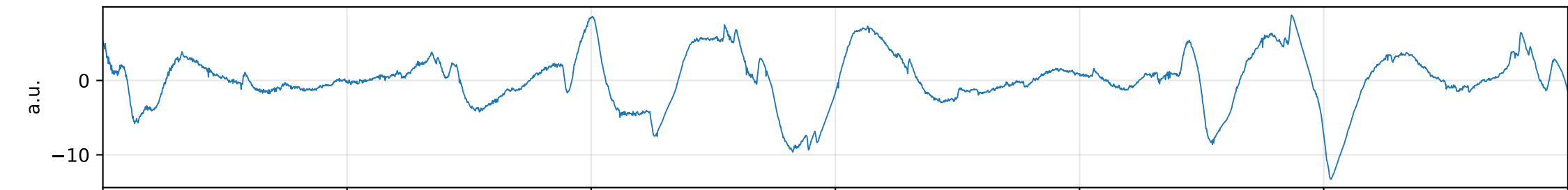
ICA component 3
