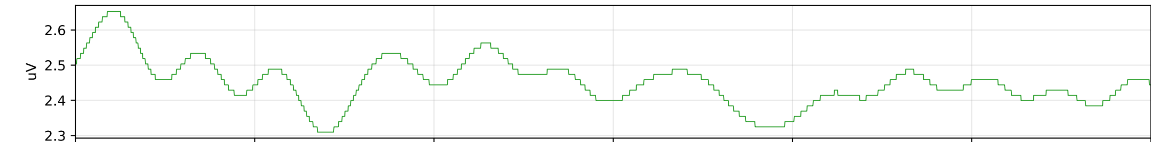
ICA component 0
