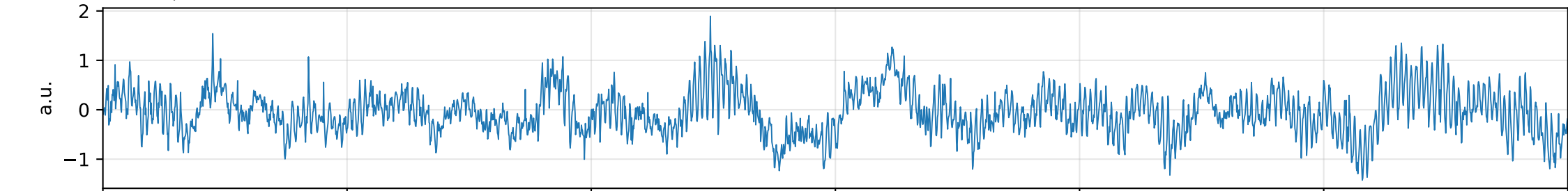
ICA component 2
